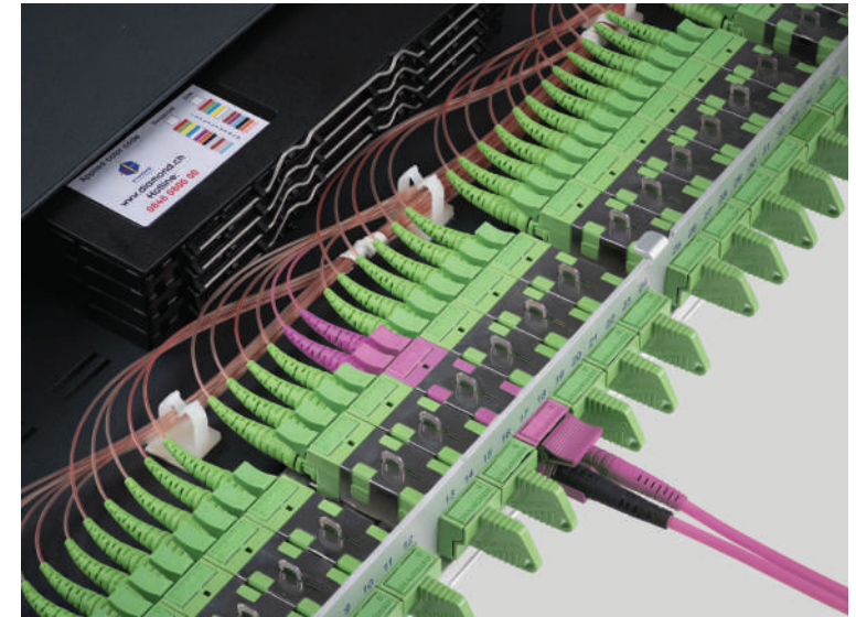
Flexpatch 1U OM4
